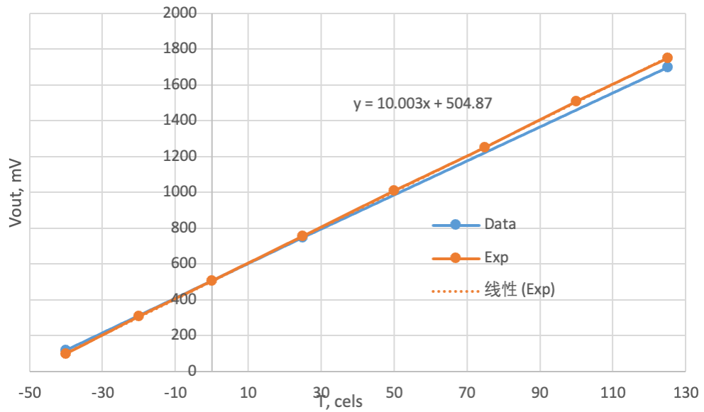
Figure 2. Characteristics of the sensor
