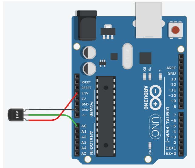
Figure 1. Thermal sensor circuit
