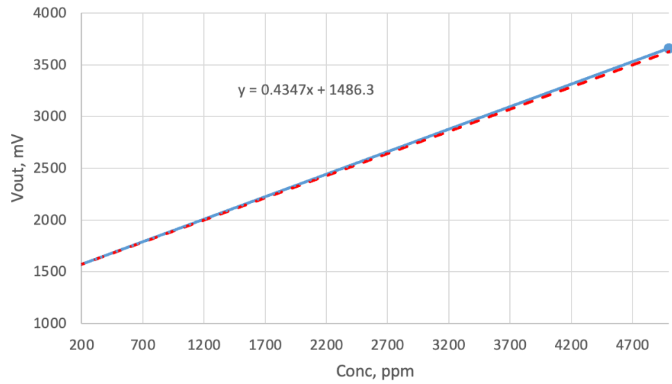
Figure 3. Gas sensor characteristic plot
