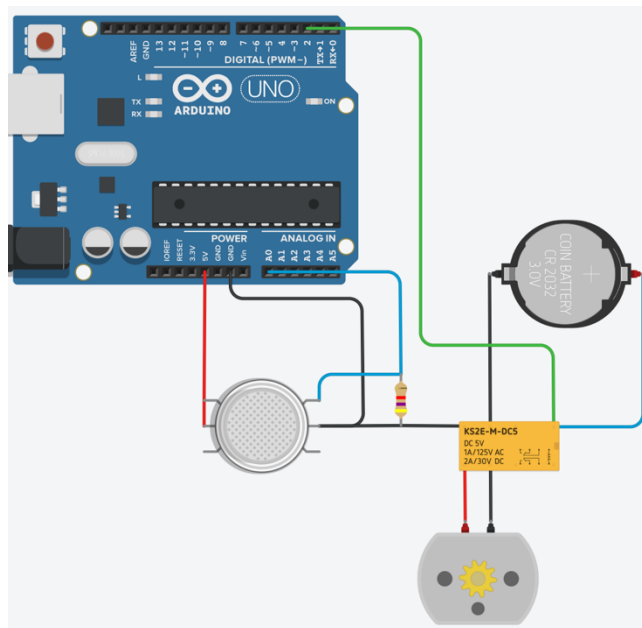
Figure 3. Gas sensor circuit (with a motor)
